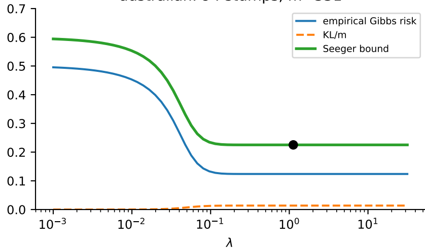
australian: 94 stumps, m=331
