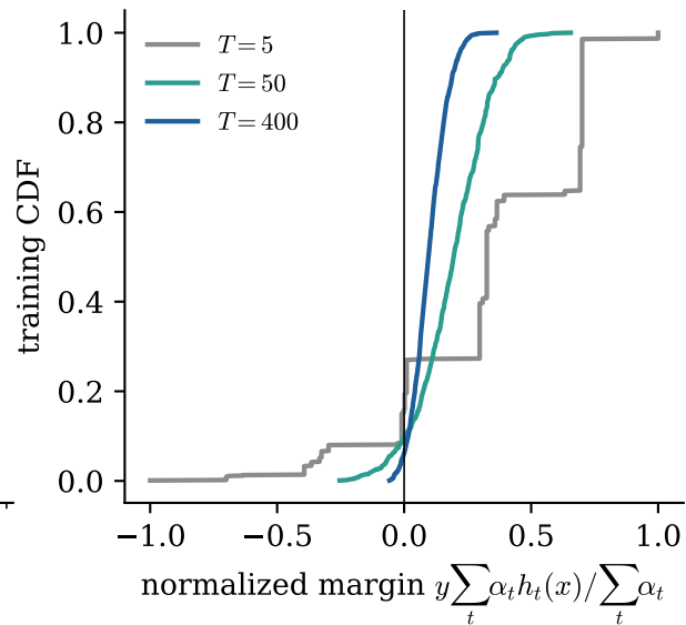
margins keep increasing
