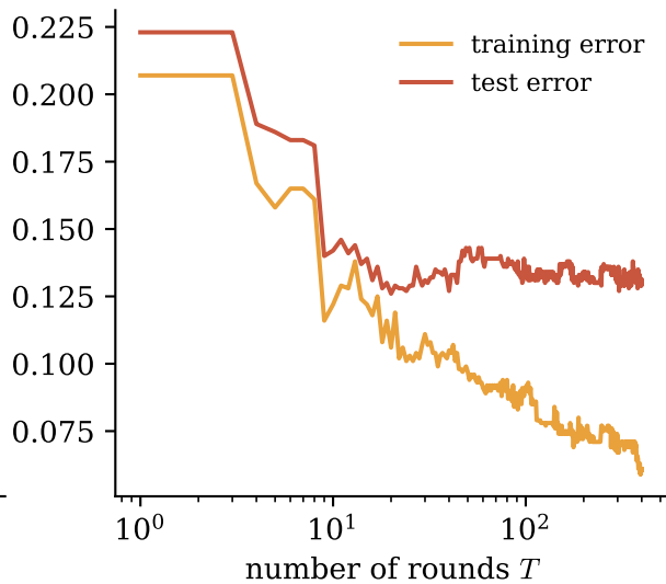
errors of the vote
