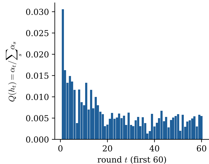
AdaBoost's vote is a distribution Q
