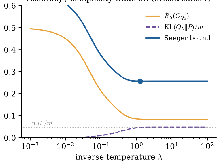
Accuracy / complexity trade-off (breast cancer)
