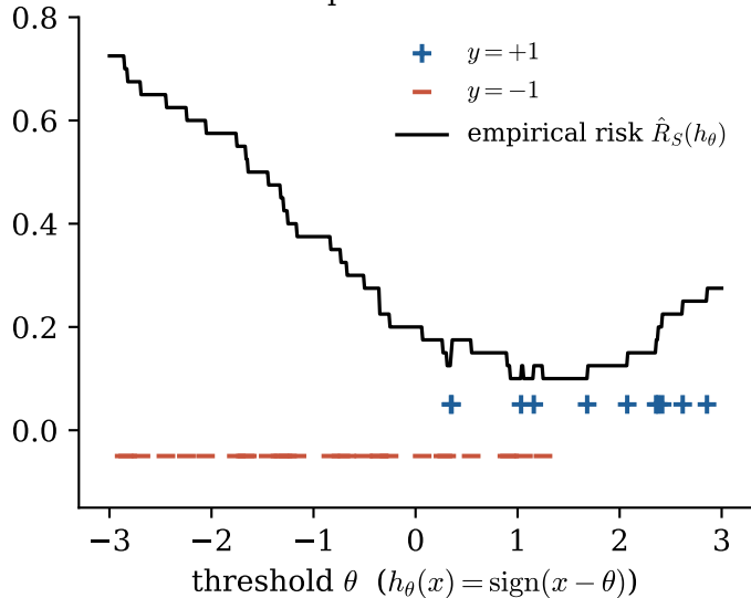
Data and empirical risk of each voter
