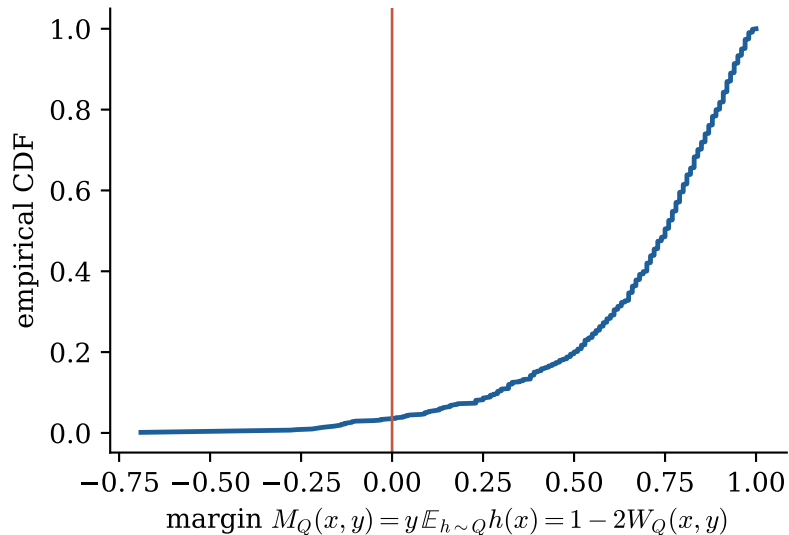
Margin distribution: R(B_Q) = \mathbb{P}(M_Q \leq 0)
