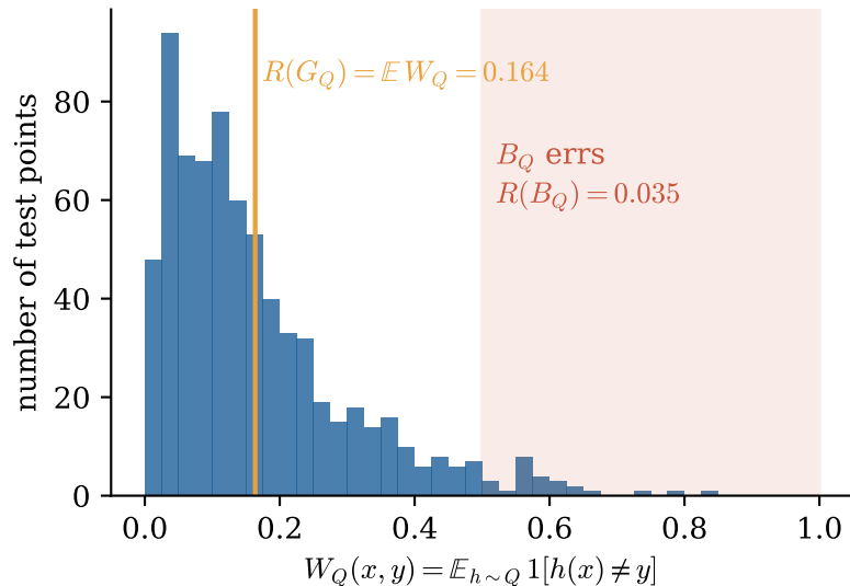
Random forest, 200 trees (digits < 5 vs \geq 5 )
