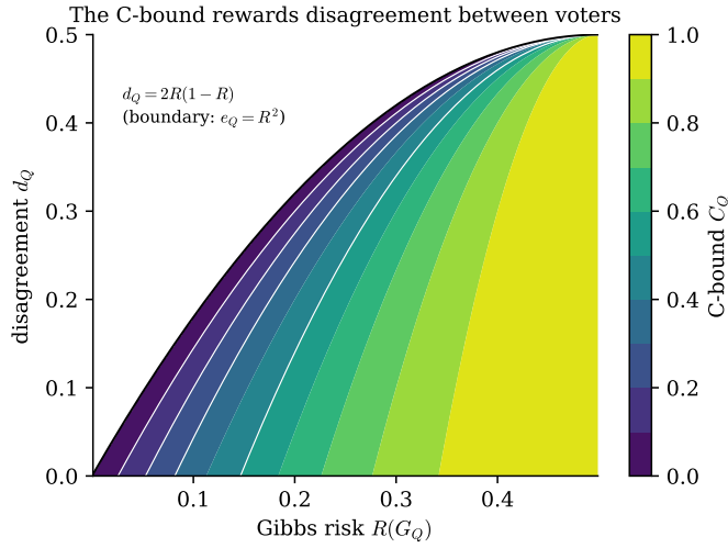
Figure 19: Value of the C-bound as a function of the Gibbs risk and the disagreement, on the feasible domain d_{\mathcal{D}} \leq 2R(1-R) . For a fixed Gibbs risk, increasing the disagreement decreases the bound: the C-bound formalizes the strength-diversity trade-off of ensemble methods (Breiman, 2001).
