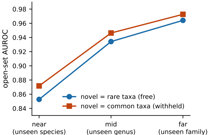
Monotone in taxonomic distance, on two novel populations chosen by opposite criteria
