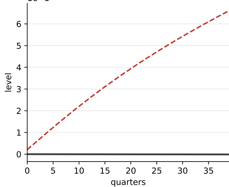
Walras residual (asset market)
