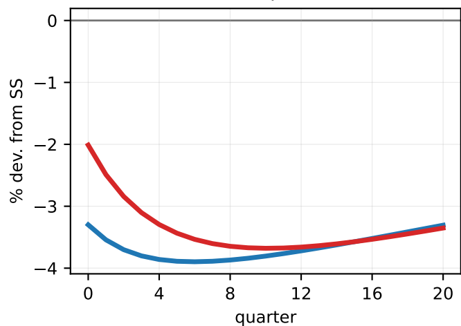
Real rate r (annualized)
