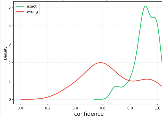
Density of confidence per status
