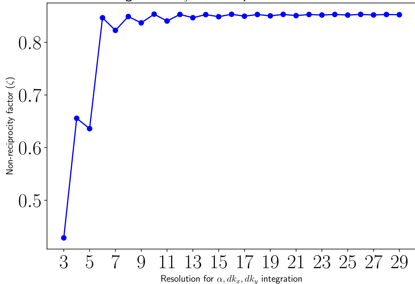
Convergence of \zeta with respect to Mesh Fineness
