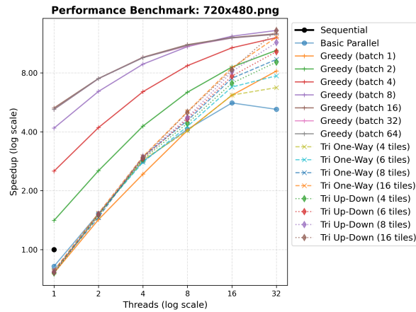
Figure 4: Speed up performance for the first image as a function of the number of threads.
