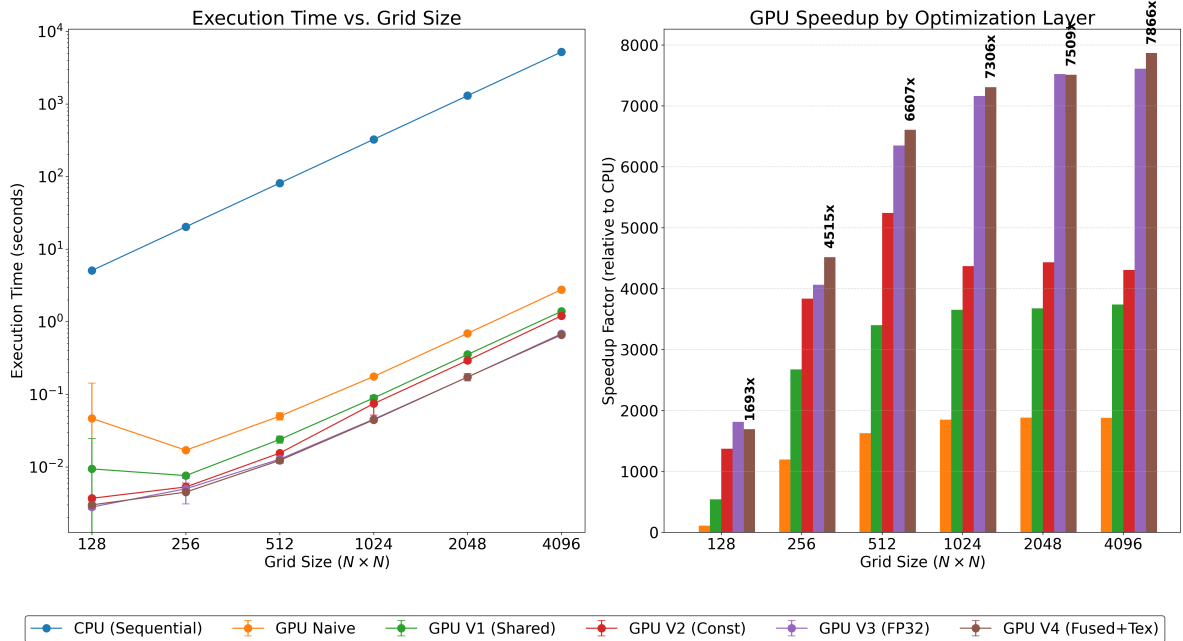
Figure 1: Performance comparison of CUDA optimization layers. Left: Log-log plot showing execution time versus grid size, highlighting the algebraic scaling advantage of the GPU implementations. Right: Grouped bar chart detailing the speedup factor of each GPU kernel relative to the sequential CPU baseline for large grid sizes.
