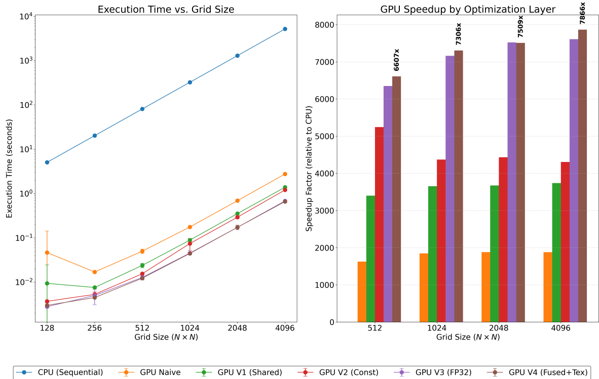
Figure 1: Performance comparison of CUDA optimization layers. Left: Log-log plot showing execution time versus grid size, highlighting the algebraic scaling advantage of the GPU implementations. Right: Grouped bar chart detailing the speedup factor of each GPU kernel relative to the sequential CPU baseline for large grid sizes.
