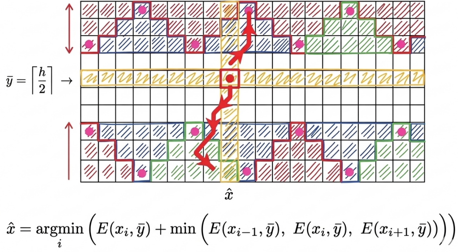
Figure 4: Bidirectional seam carving synchronization at the image midpoint \bar{y} . The upward and downward wavefronts (red arrows) converge at the central row, where the optimal transition point \hat{x} is determined by minimizing the combined energy from both computed halves.
