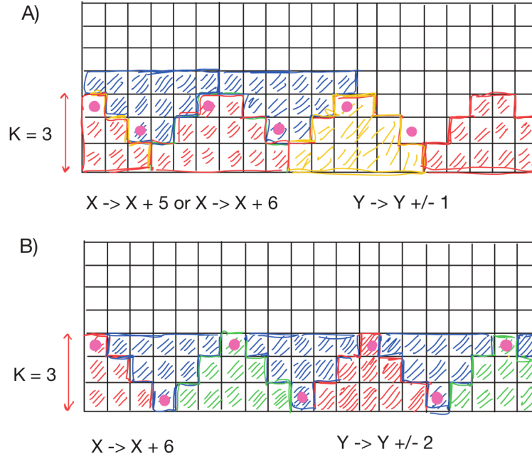
Figure 5: Comparison of wavefront tiling strategies for parallel seam carving for a tile height of 3.
