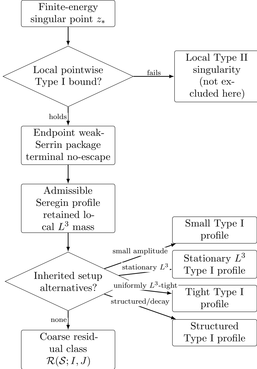
FIGURE 2. Rendered entry tree. Local pointwise Type I enters the setup admissible Seregin package through endpoint weak Serrin estimates and terminal no-escape. If the bound fails, the point belongs to the local Type II alternative, which is not excluded here.
