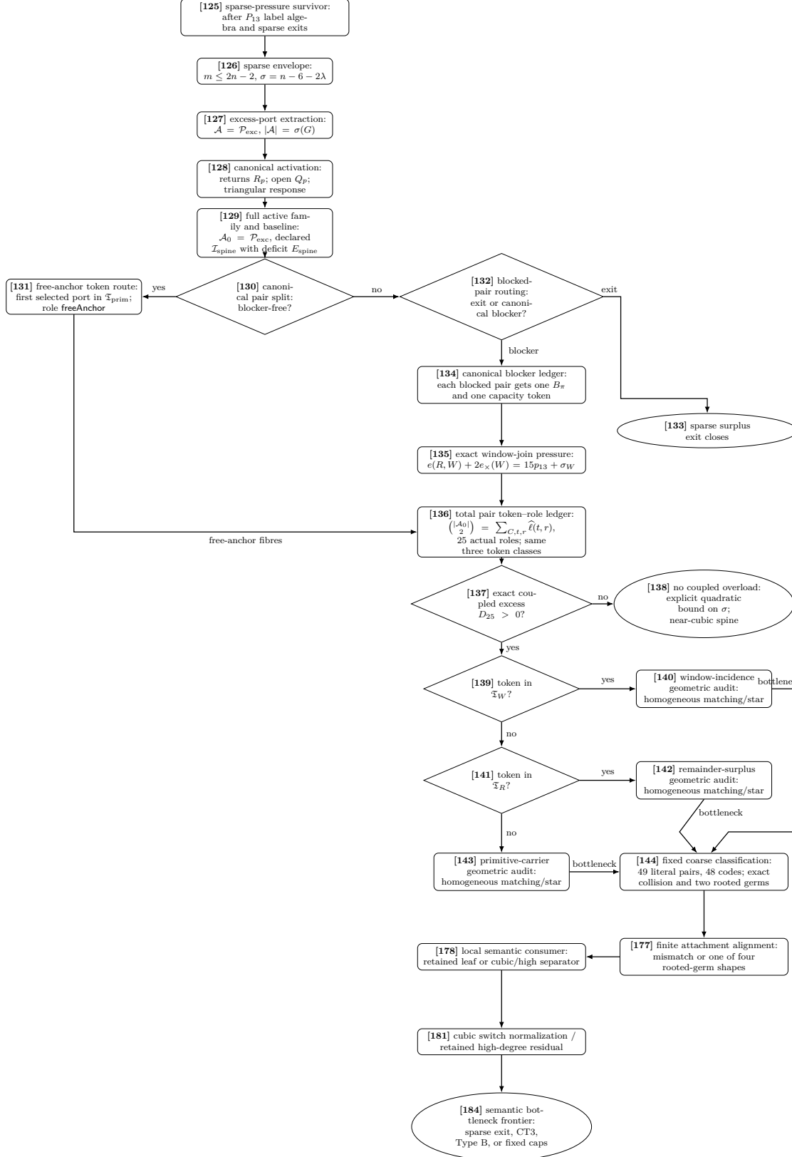
Figure 10: Proof-dependency diagram, Part X. This panel expands the sparse non-near-cubic branch [20]. Nodes [126]–[128] build the full active surplus family, and node [129] records the separate baseline-demand definition with its exact deficit. Node [130] performs the canonical blocker split. At [131], every blocker-free pair is assigned to its first selected surplus port, which is already a primitive token, with the distinct role freeAnchor . Blocked pairs pass through [132]–[134] and receive their canonical capacity token. The two routes join at [136], where the 25 token–role labels partition the complete scheduled-pair family without double counting. Node [137] is the exact coupled CT9 definition of D_{25} , with its explicit quadratic bound on \sigma(G) for near-cubic spines. Node [139] checks for a token in \mathcal{I}_W , leading to the window-incidence geometric audit [140]. If not, [141] checks for a token in \mathcal{I}_R , leading to the remainder-surplus geometric audit [142]. Both [140] and [142] lead to the fixed coarse classification [144] via a bottleneck. [143] is the primitive-carrier geometric audit, also leading to [144] via a bottleneck. [144] leads to finite attachment alignment [177], then local semantic consumer [178], then cubic switch normalization [181], and finally the semantic bottleneck frontier [184].
