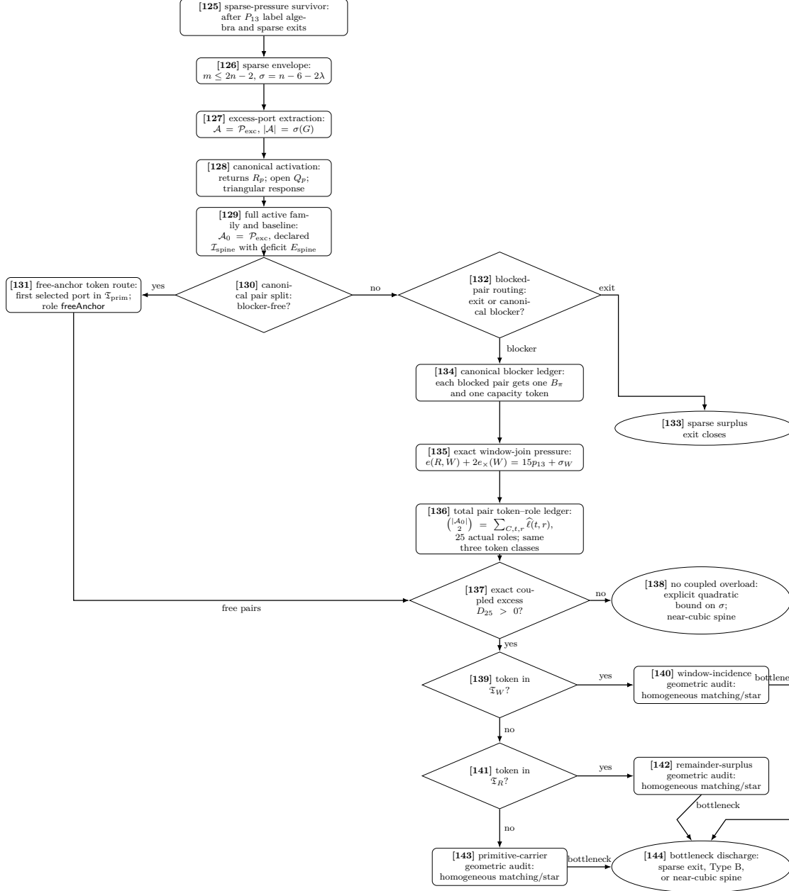
Figure 10: Proof-dependency diagram, Part X. This panel expands the sparse non-near-cubic branch [20]. Nodes [126]–[128] build the full active surplus family, and node [129] records the separate baseline-demand definition with its exact deficit. Node [130] performs the canonical blocker split. At [131], every blocker-free pair is assigned to its first selected surplus port, which is already a primitive token, with the distinct role freeAnchor . Blocked pairs pass through [132]–[134] and receive their canonical capacity token. The two routes join at [136], where the 25 token–role labels partition the complete scheduled-pair family without double counting. Node [137] is the exact coupled CT9 decision of Proposition 3.59; it consumes the literal pair count \binom{\sigma(G)}{2} , not a Boolean-realization estimate. If D_{25} = 0 , the explicit quadratic surplus bound routes to [138]. If D_{25} > 0 , CT9 returns an actual overloaded token–role fibre. Nodes [139] and [141] inspect the literal constructor of that token and route it to the window-incidence, remainder-surplus, or primitive-carrier geometric audit [140], [142], [143]. A free-anchor fibre lies in the primitive class and is a literal same-first-port star. Node [144] consumes the finite attachment and local-separator support internally and returns exactly the original sparse-exit, Type B, or near-cubic-spine alternative.
