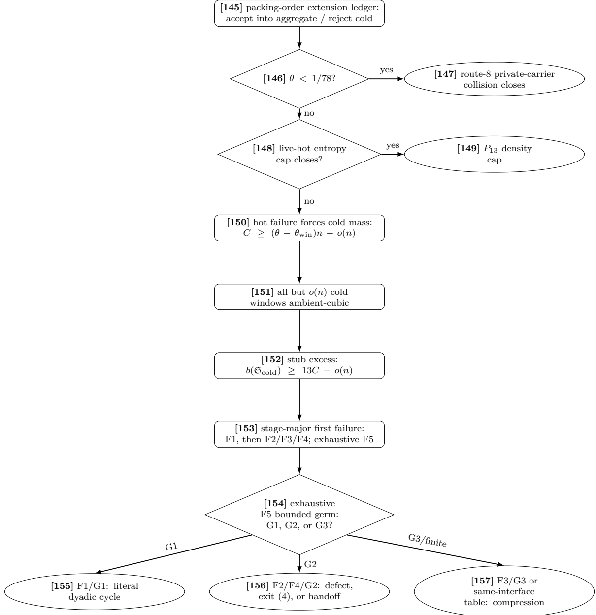
Figure 11: Proof-dependency diagram, Part XI. This panel preserves the original hot/cold P_{13} -window topology behind nodes [22]–[24]. If \theta < 1/78 , route 8 closes at [147]. Otherwise the hot entropy cap yields [149] or a linear unpaid cold family [150], followed by the near-cubic and stub-excess stages [151]–[152]. Node [153] contains the graph-owned local attachment, return, component, and D1–D7 first-failure computations; only exhaustive F1–F4 absence enters the germ trichotomy [154] as F5. The three original consumers remain [155], [156], and [157].
