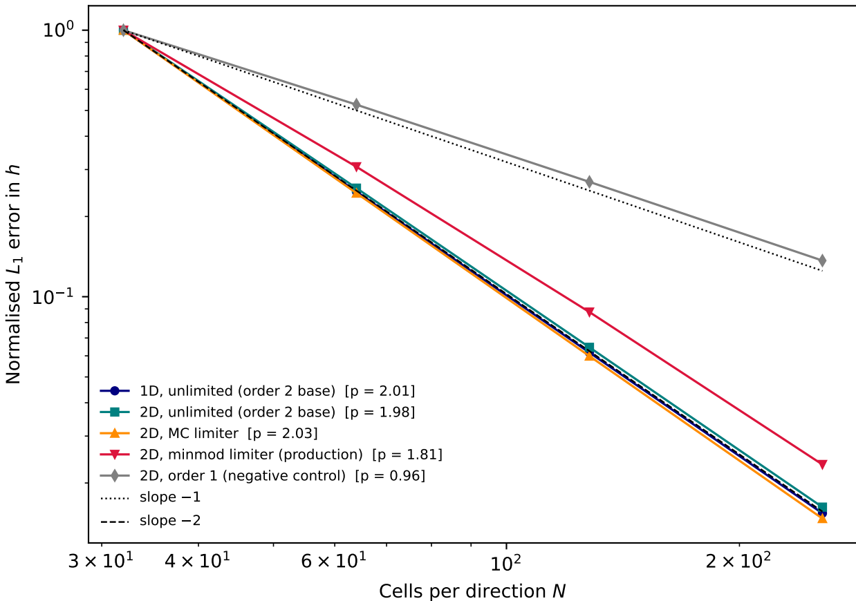
Formal order of accuracy (manufactured solution)
