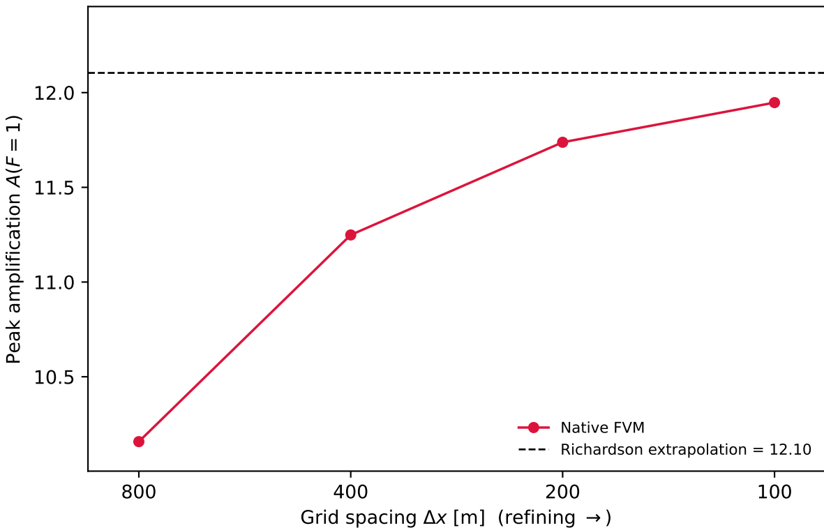
Mesh convergence of the resonant peak
