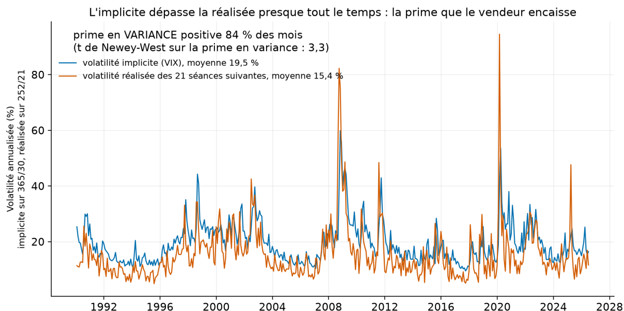
Fig. 2. – Prime de variance
