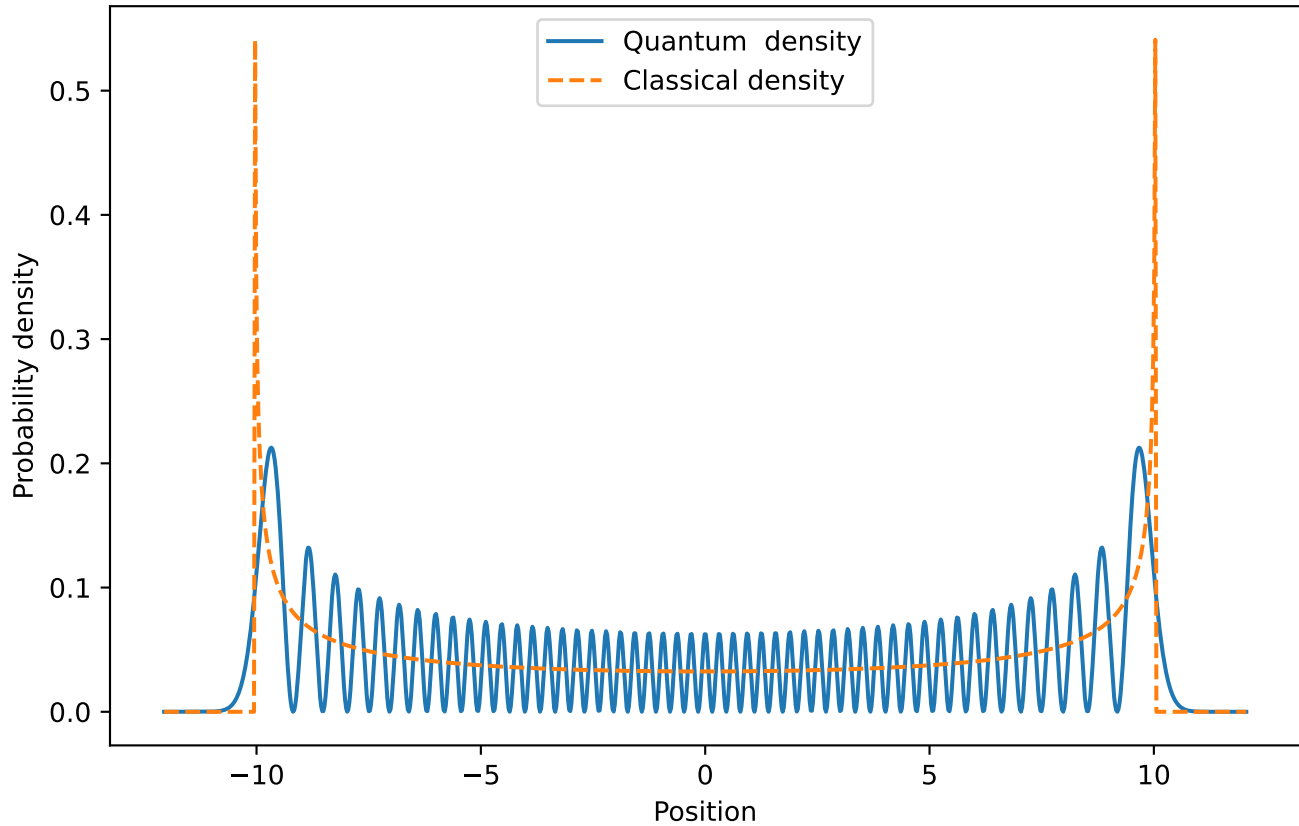
Quantum vs Classical Probability Density (n=50)
