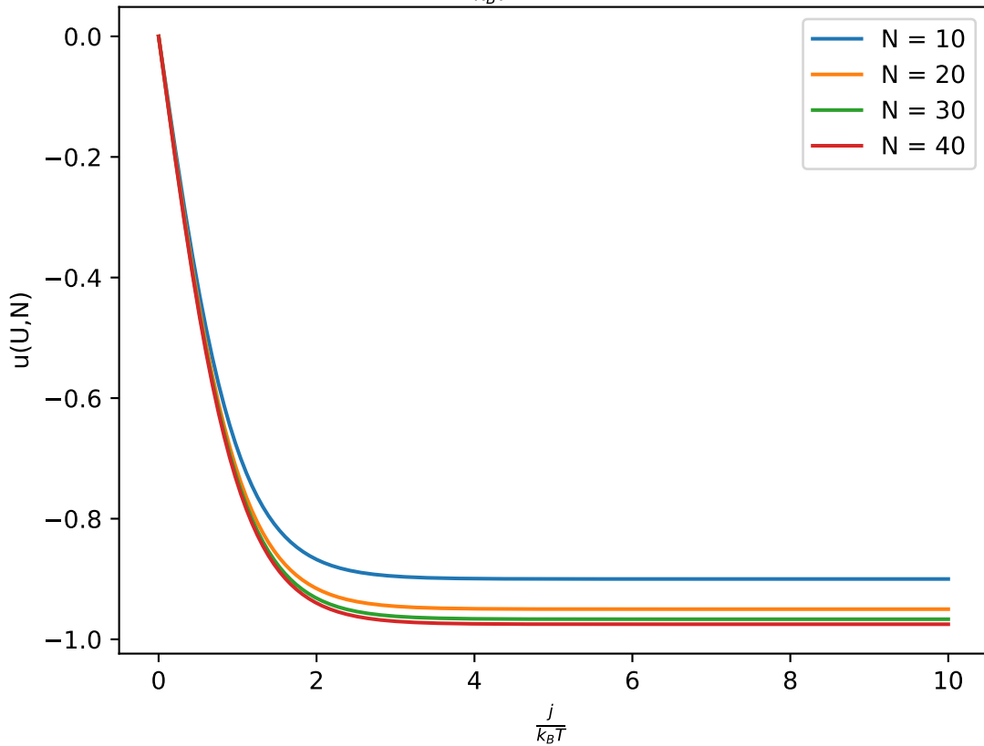
Plot of " u(U, N) \times \frac{j}{k_B T} " for different values of N
