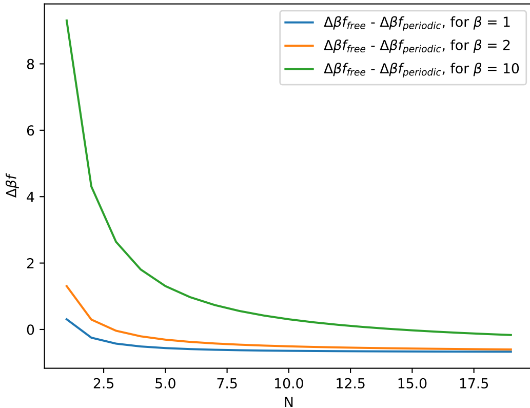
Difference between periodic and free Boundary conditions as a function of N
