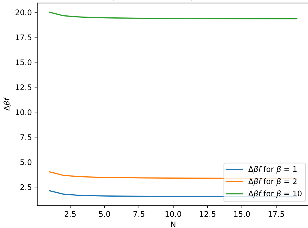
\Delta\beta f as a function of N in periodic Boundary conditions
