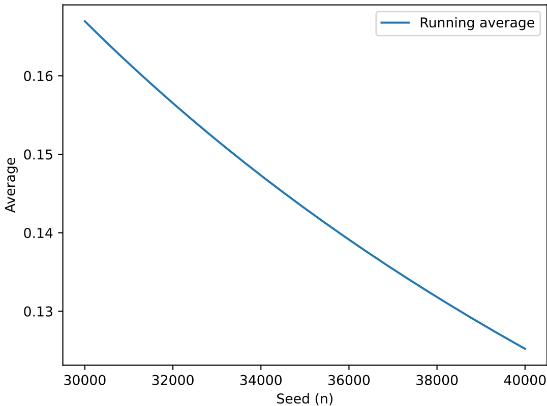
Running average of Pseudo Random numbers, n \in [30000, 40000]
