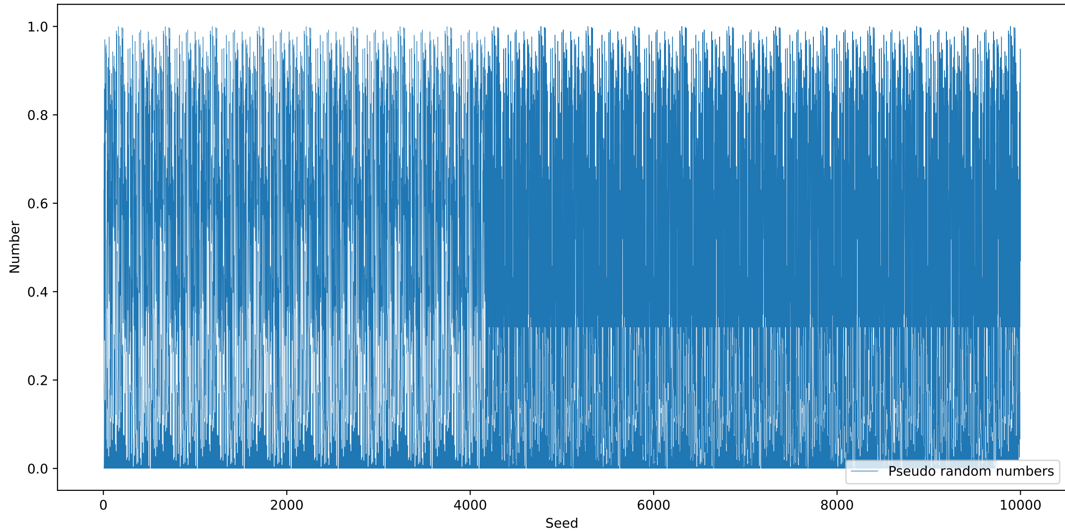
Time series of generated pseudo random numbers
