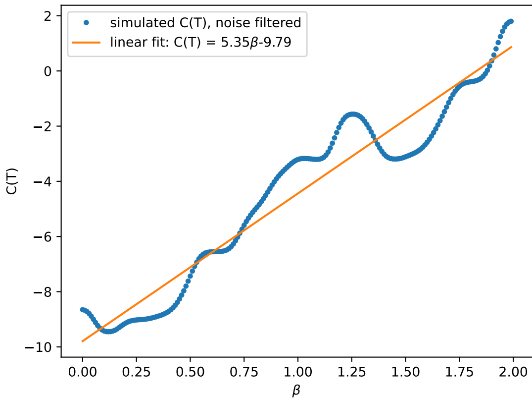
Heat capacity C(T) in function of \beta
