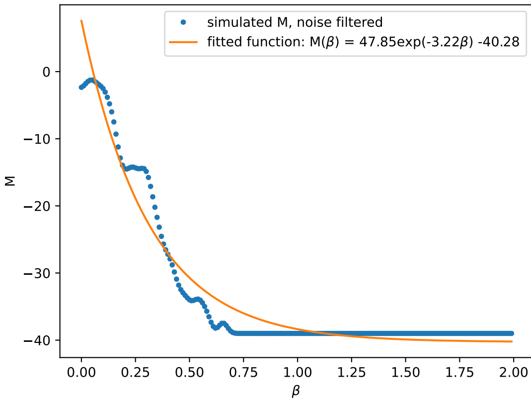
Magnetization M in funtion of \beta
