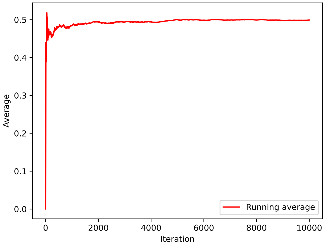
Running average of 10000 Pseudo Random numbers
