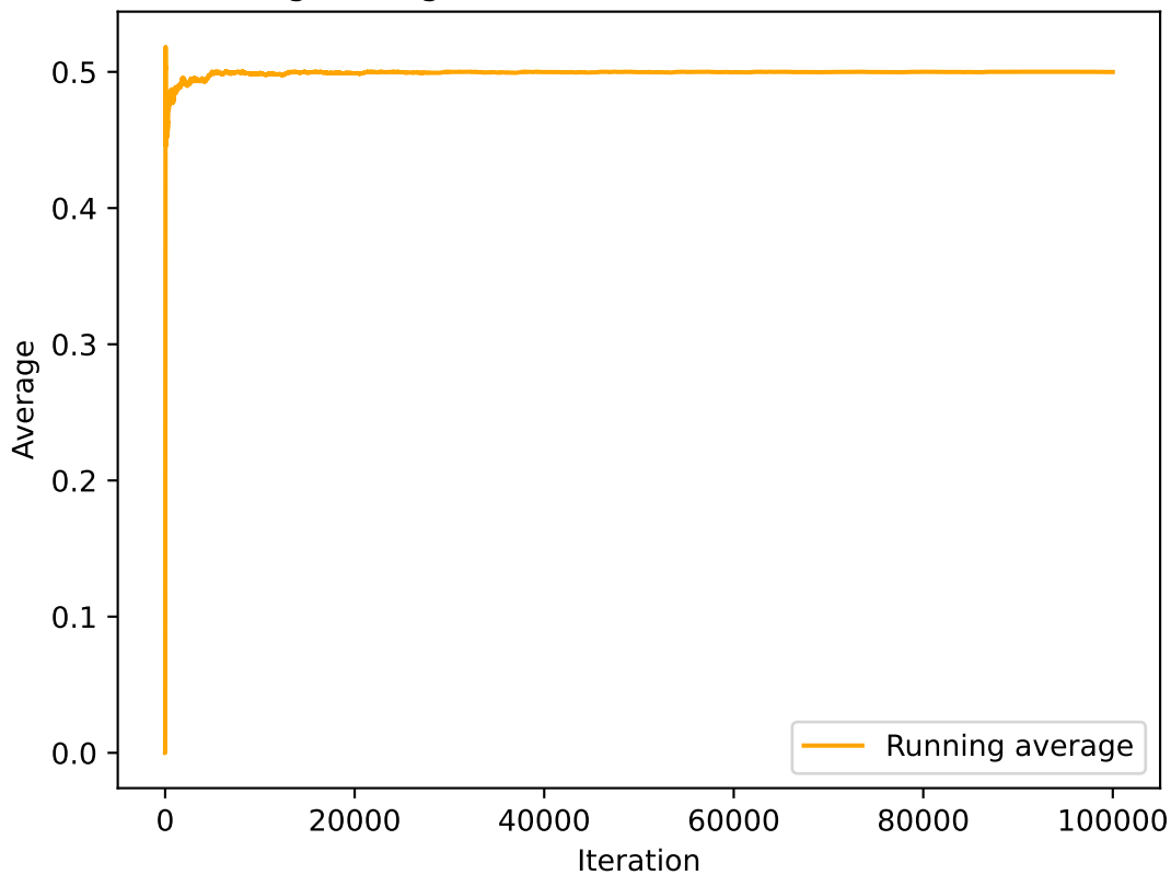
Running average of 100000 Pseudo Random numbers
