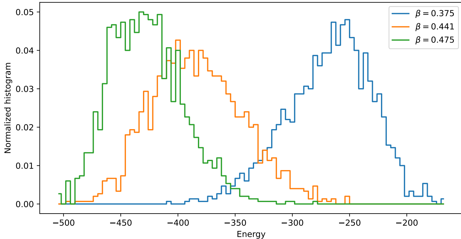
Energy histograms used for WHAM
