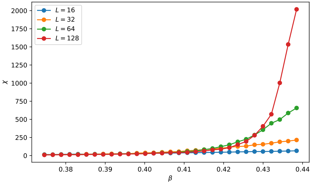
Susceptibility versus \beta
