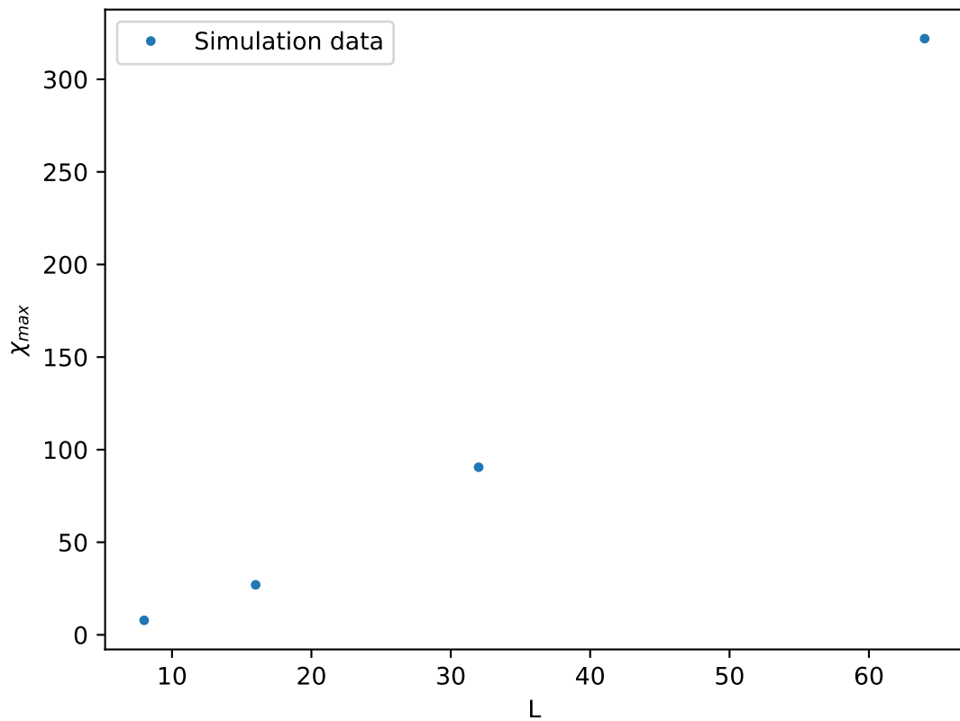
\chi_{max} in function of L
