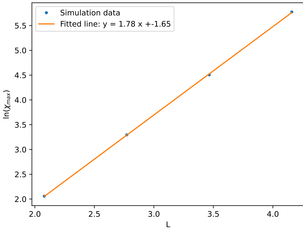
\ln(\chi_{max}) in function of \ln(L)
