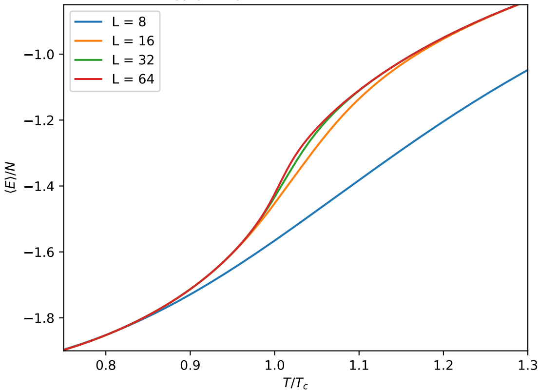
Energy per spin for different lattice sizes
