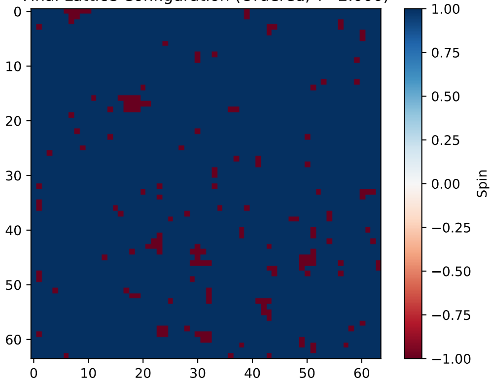
Final Lattice Configuration (Ordered, T=2.000 )
