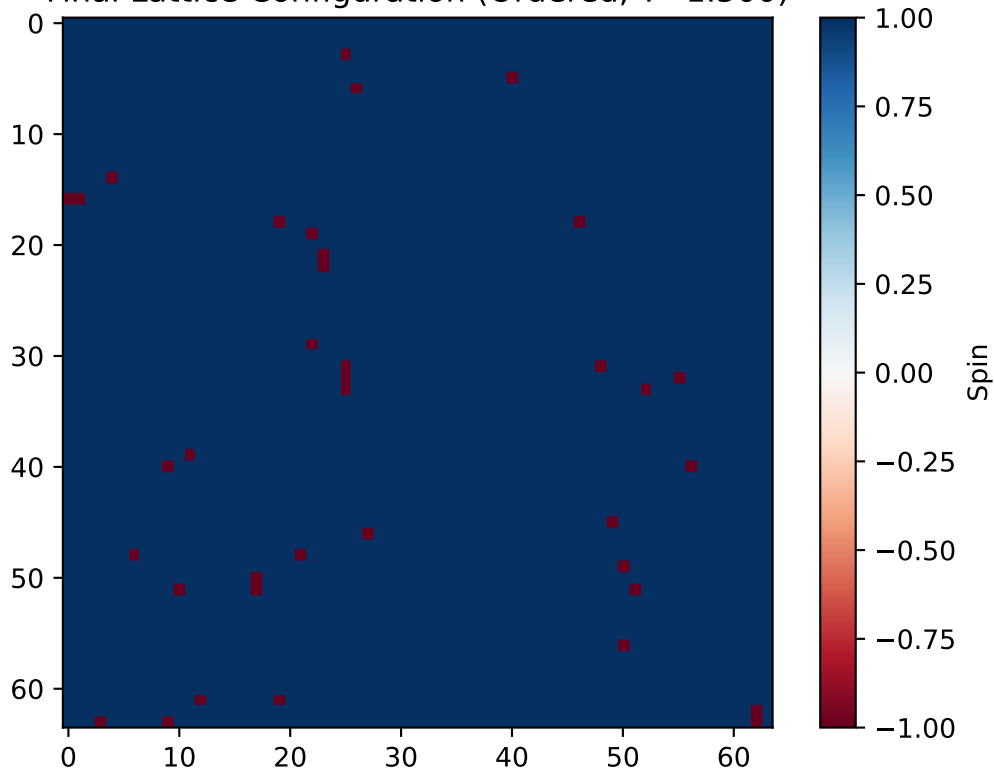
Final Lattice Configuration (Ordered, T=1.500 )
