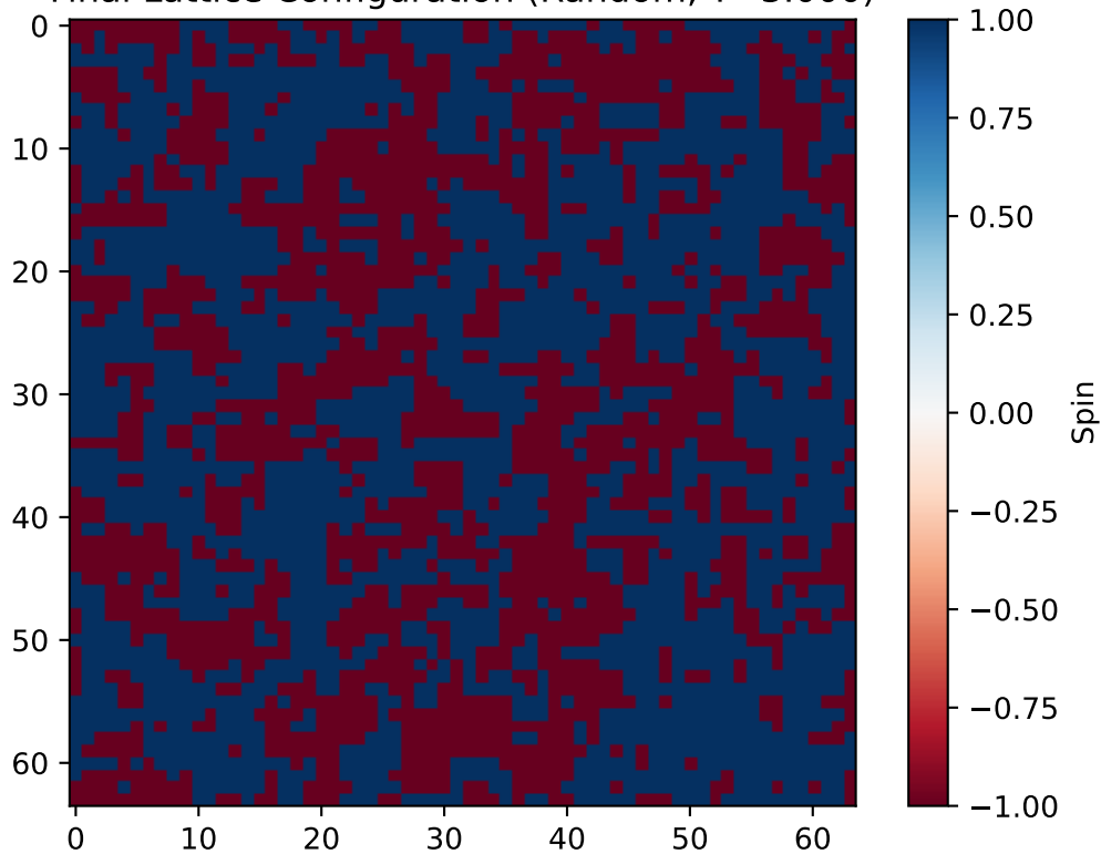
Final Lattice Configuration (Random, T=3.000 )
