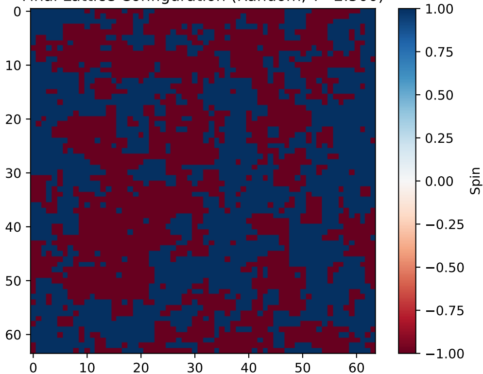
Final Lattice Configuration (Random, T=2.500 )
