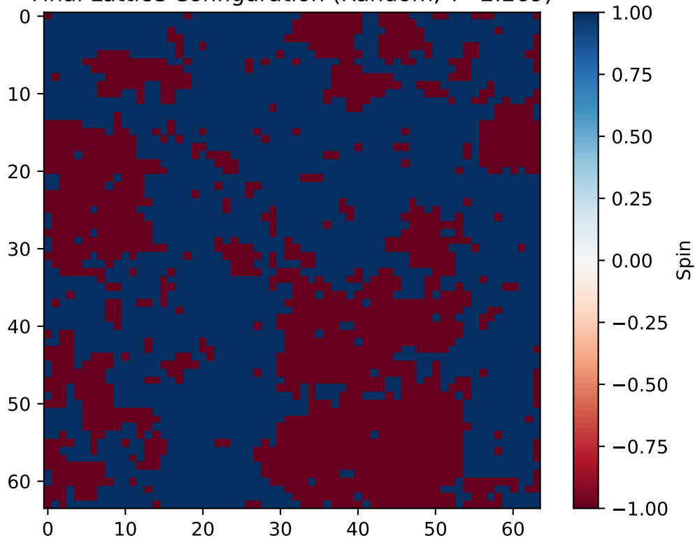
Final Lattice Configuration (Random, T=2.269 )
