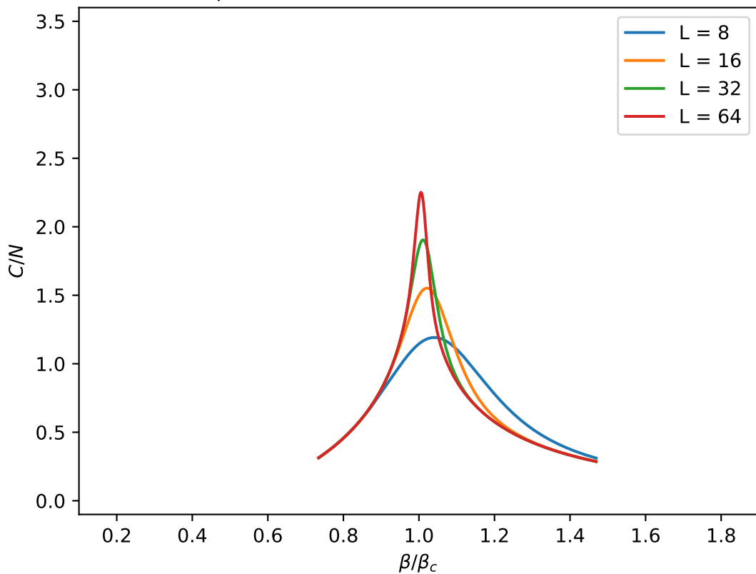
Specific Heat for different lattice sizes
