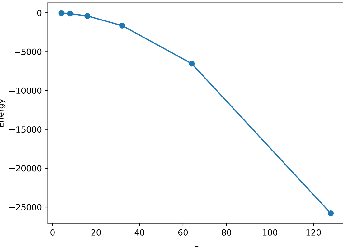
Energy vs L at \beta c
