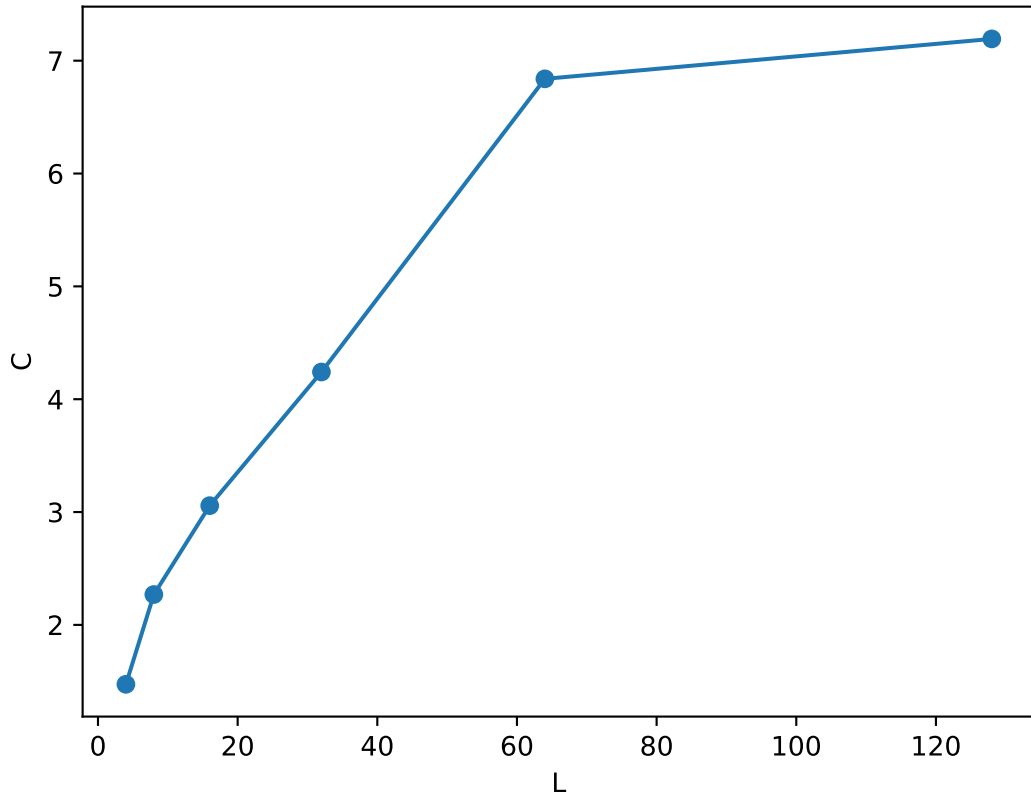
Specific Heat vs L at \beta_c
