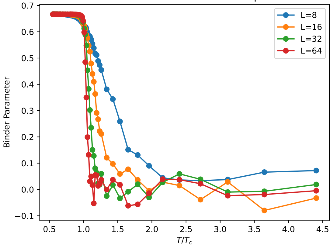
Binder Parameter vs Normalized Temperature
