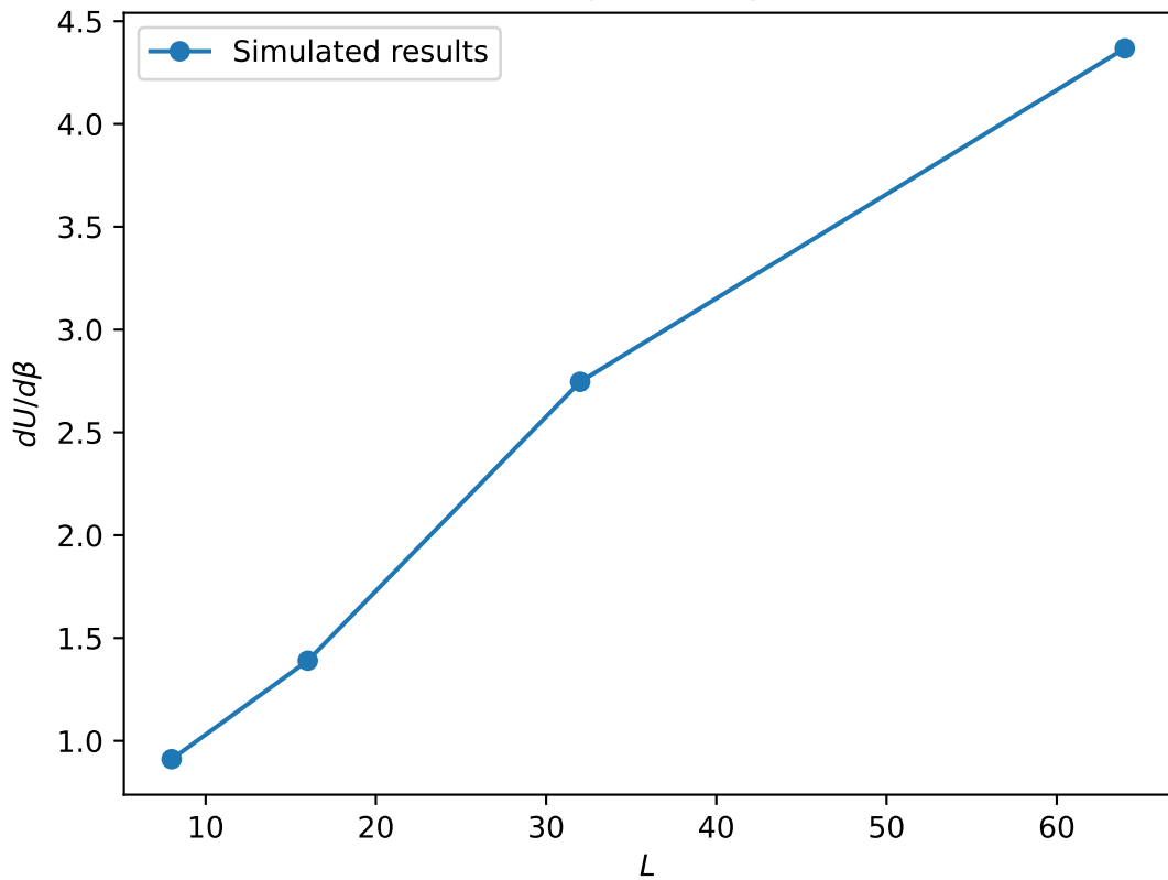
dU/d\beta vs L at \beta_c
