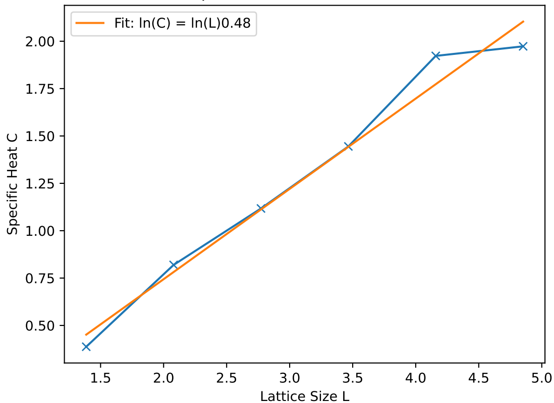
Specific Heat vs Lattice Size
