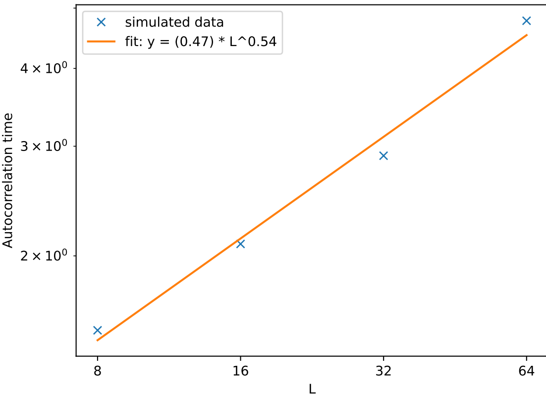
Autocorreletaion time vs Lattice size
