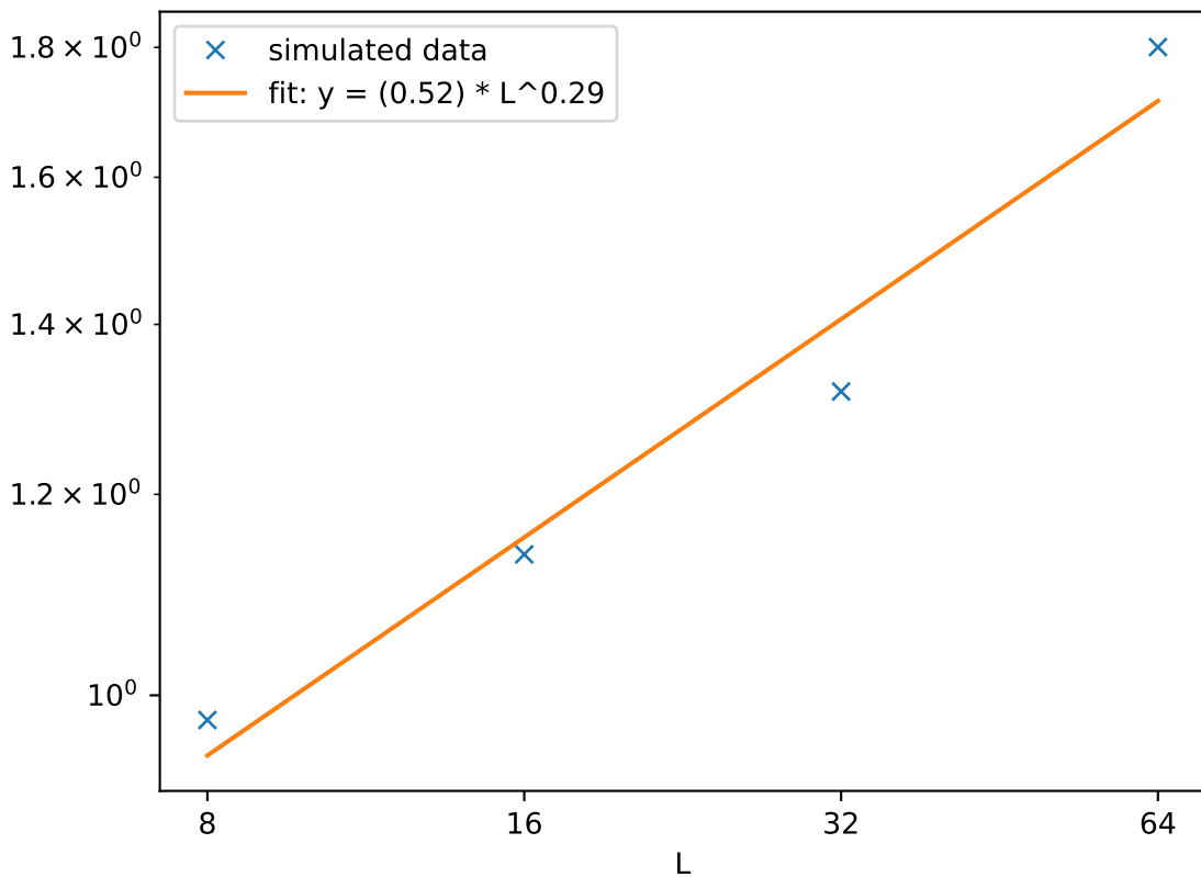
Autocorreletaion time vs Lattice size (rescaled)
