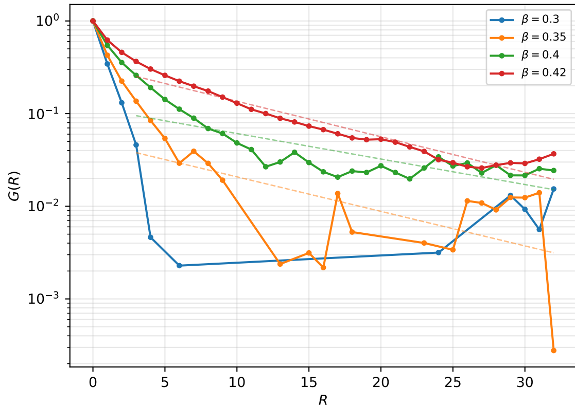
Standard estimator
